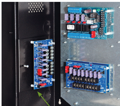
BR1 with sub-assembly (not included) mounted to side wall of Trove Enclosure.
