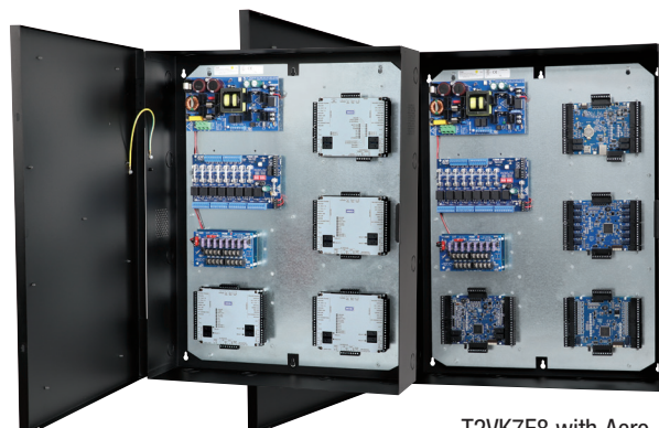
T2VK7F8 with Aero boards in cases
