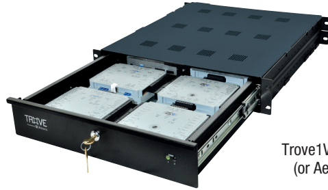
Trove1V1R with Altronix power supply and sub-assemblies and three (3) HID VertX® (or Aero™) access controllers
