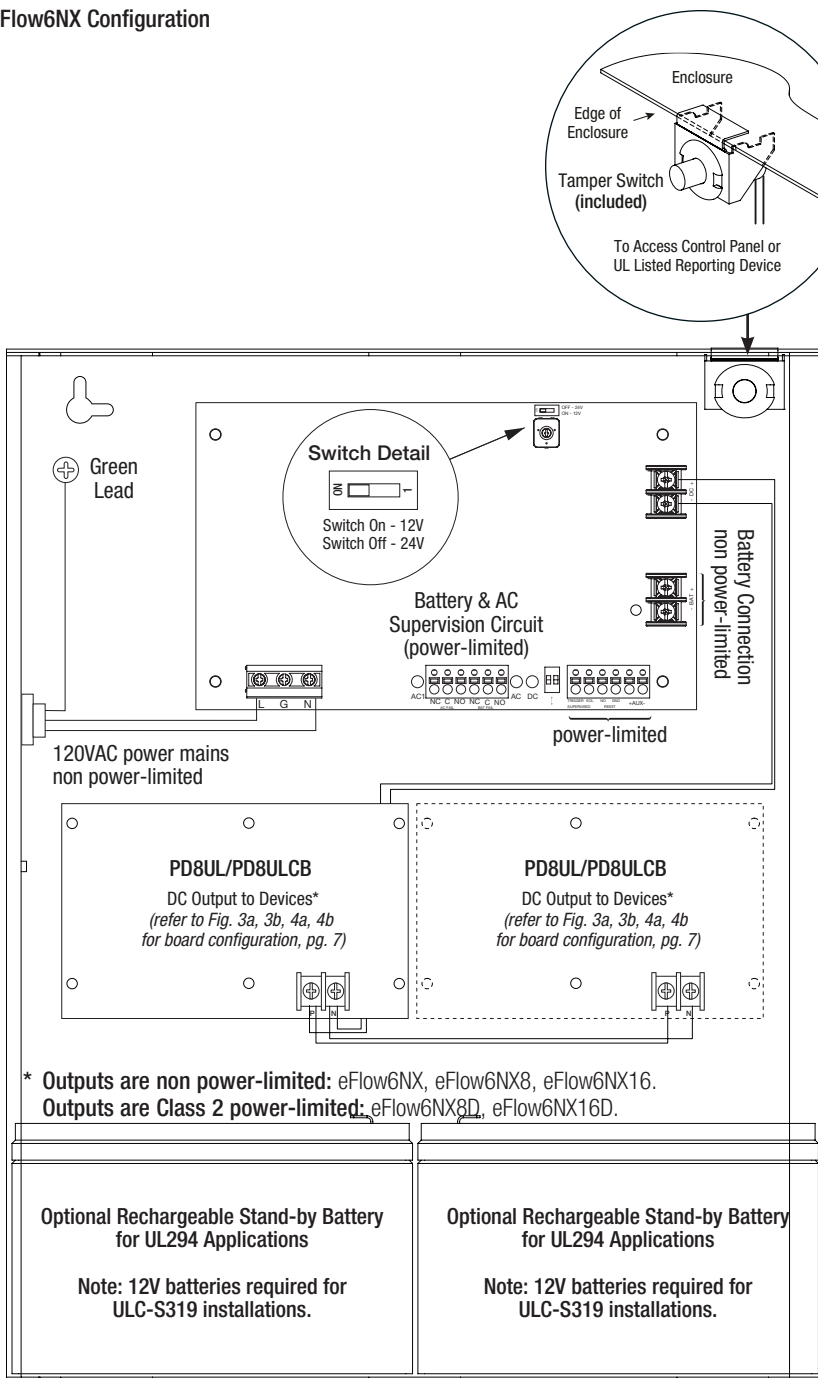
Fig. 7 - eFlow6NX Configuration
