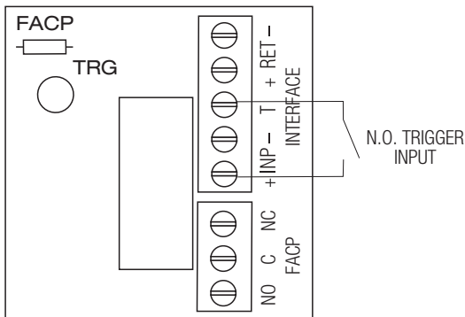
Fig. 7 Normally Open: Non-Latching FACP trigger input:
